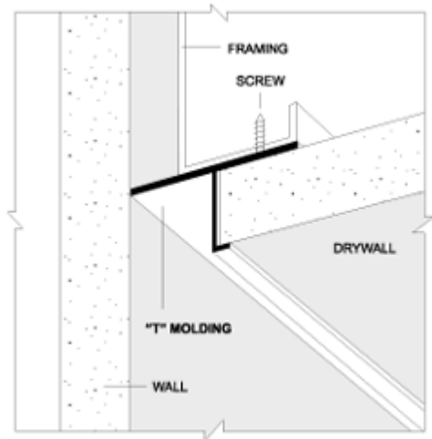
INSTALLATION DETAIL : Perspective
