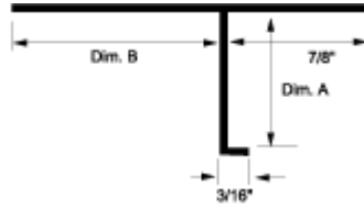
PRODUCT DETAIL : Full Scale
