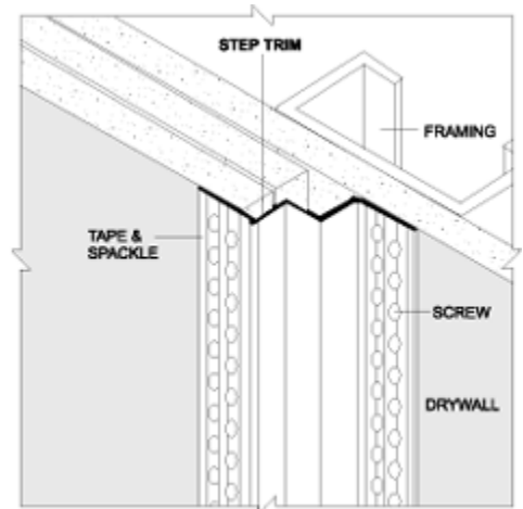
INSTALLATION DETAIL : Perspective
