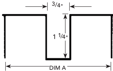
GLAZING TRACK
