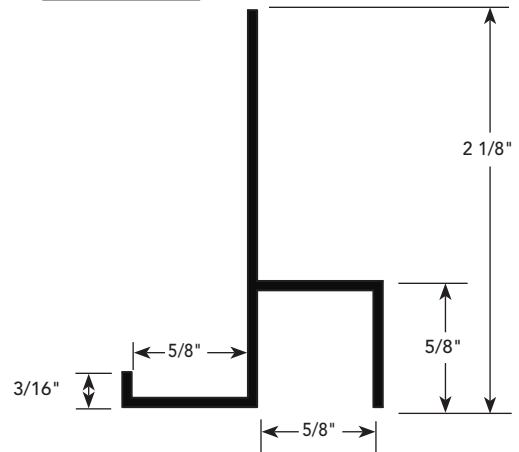
PART NUMBER 1054
