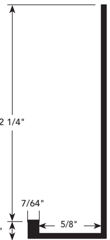
PART NUMBER 1262
