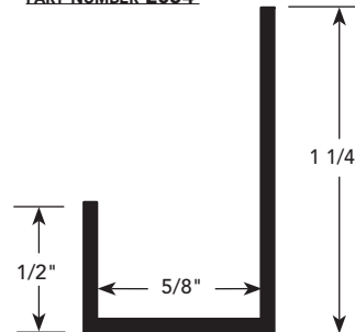
PART NUMBER 2054
