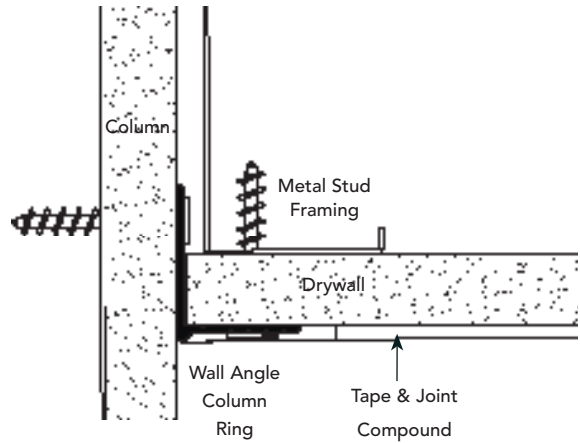
CROSS SECTION - ACOUSTICAL/DRYWALL
