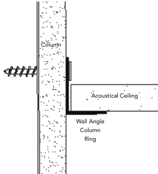
CROSS SECTION - ACOUSTICAL/DRYWALL
