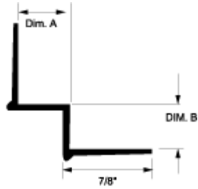
PRODUCT DETAIL : Full Scale
