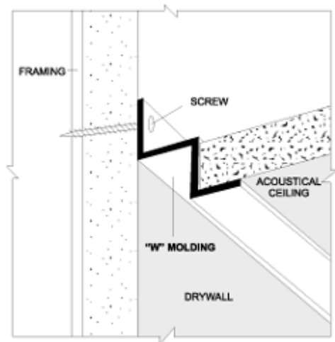
INSTALLATION DETAIL : Perspective
