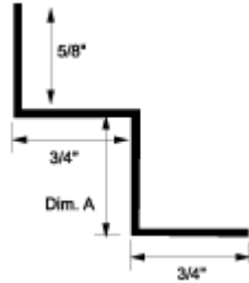
PRODUCT DETAIL : Full Scale
